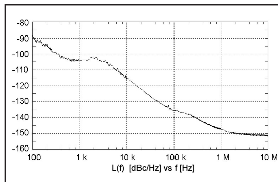
Typical SSB Phase Noise at 1 GHz, phase noise optimized >10 kHz offset
