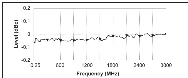
Typical flatness at 0 dBm
